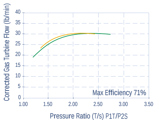
GT35, 84 trim, 1.18 A/R GT35, 84 trim, 1.05 A/R
