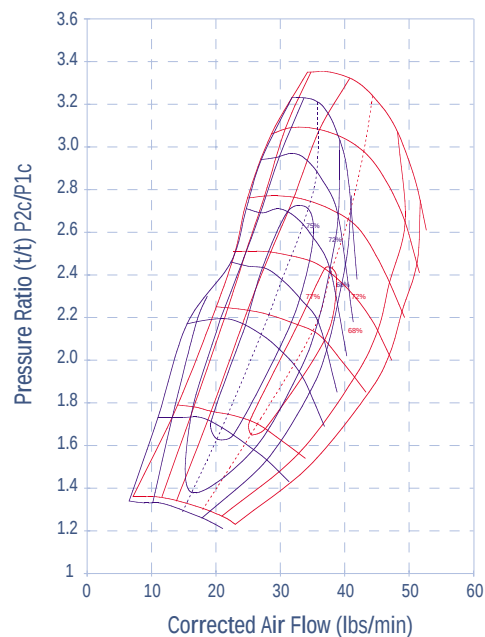
GT35 71mm, 52 trim, 0.50 A/R GT35 76mm, 52 trim, 0.50 A/R
