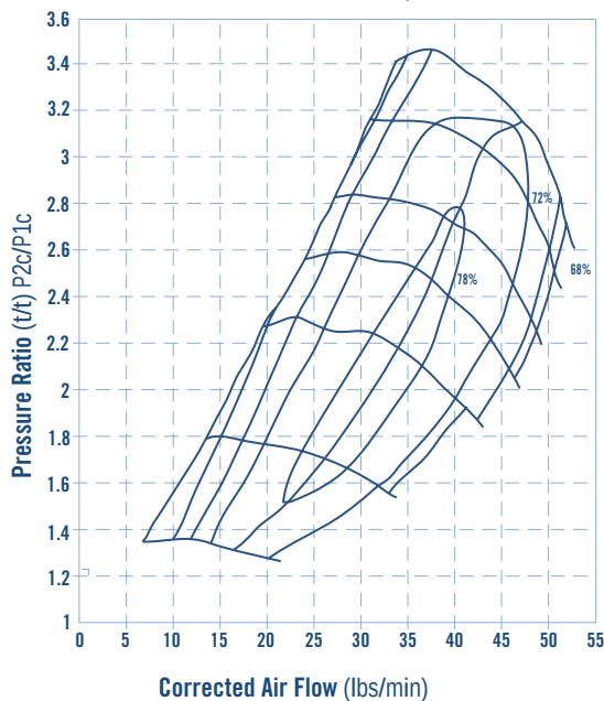
GT30R 76.2mm 56 trim, 0.60 A/R
